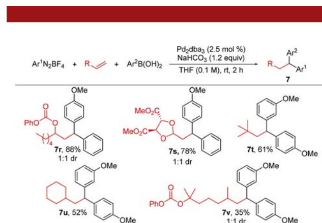
Figure 3. Scope of 1,1-diarylation of various alkenes.
